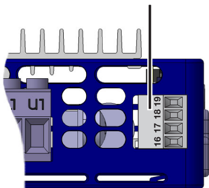
(RS422/485 Modbus)
